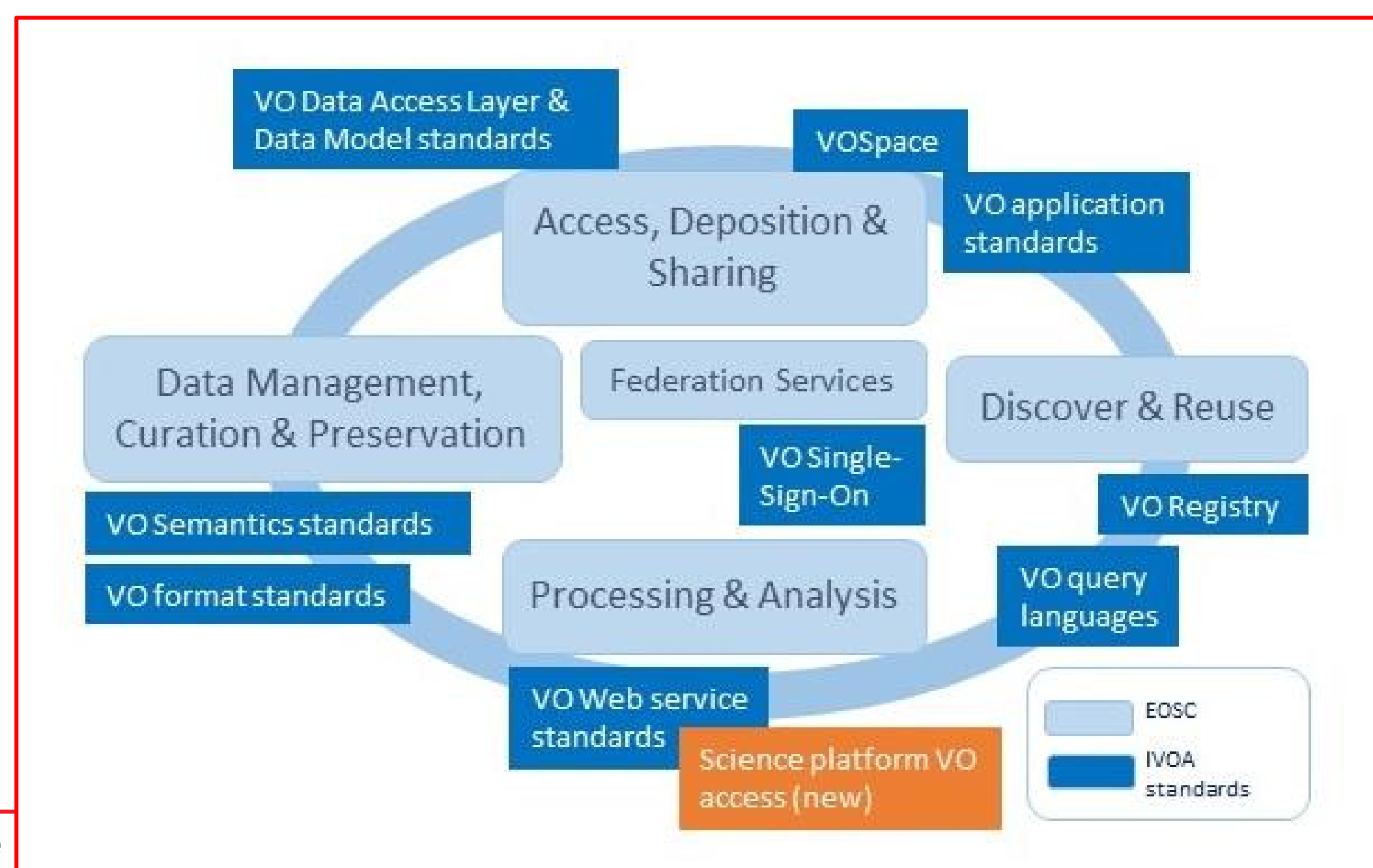
VO mapping onto the EOSC data lifecycle
